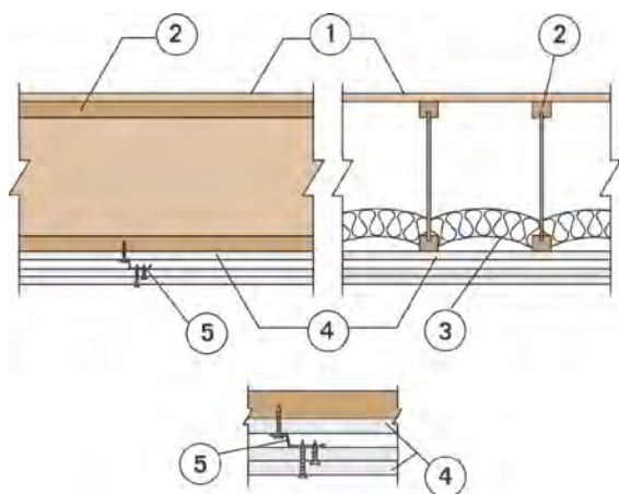
FIGURE 4G—ASSEMBLY G (Two-hour Fire-resistance-rated Roof-ceiling or Floor-ceiling Assembly):
