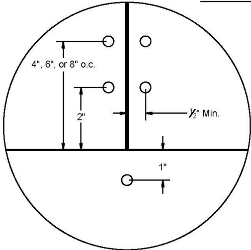
1. Two-Span offset of Seams w/o Blocking
