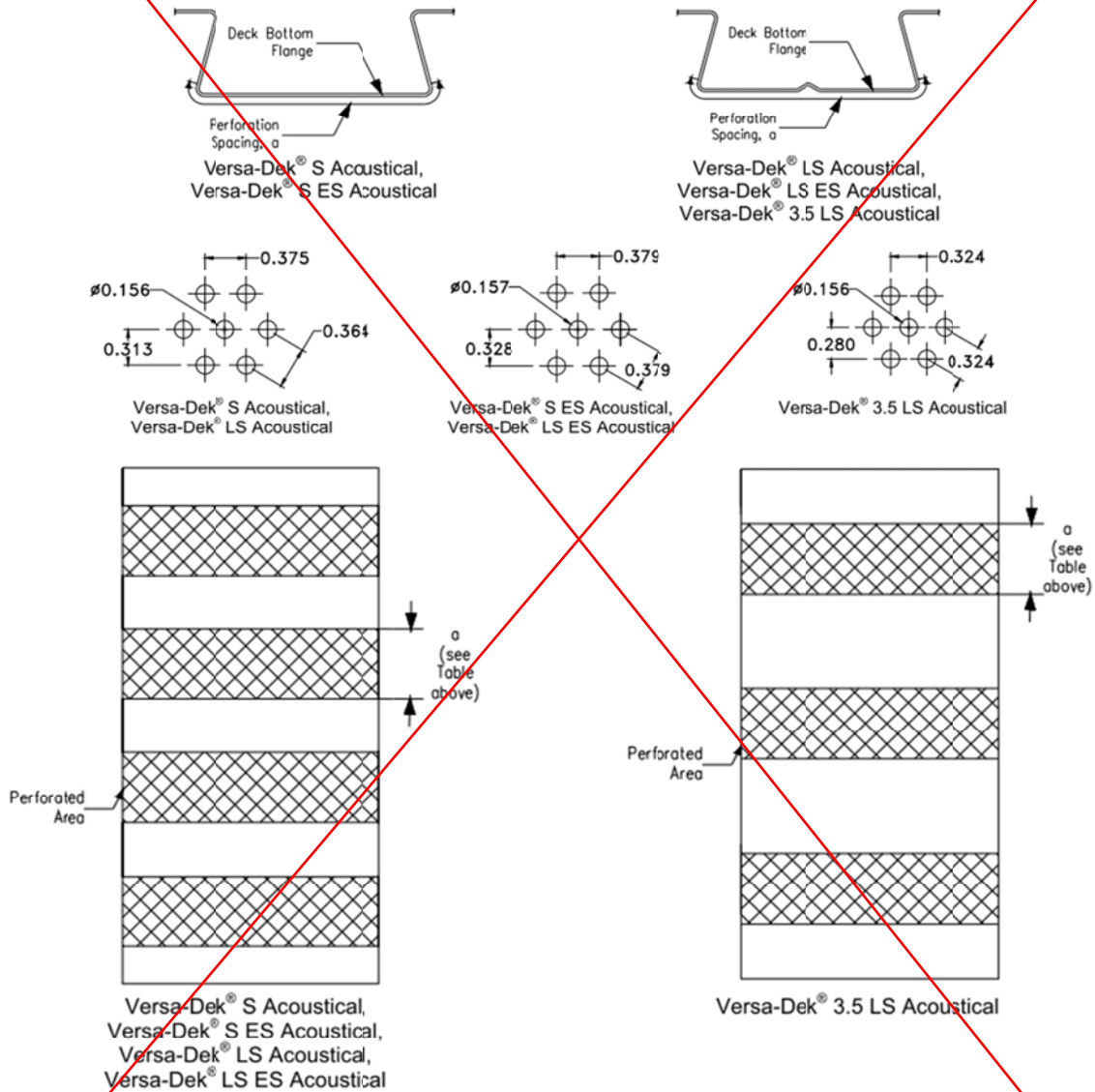
FIGURE 2—PERFORATION PATTERNS OF VERSA-DEK ACOUSTICAL PROFILES
