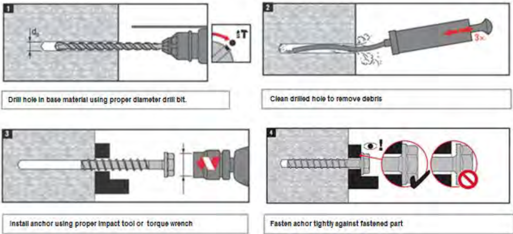
FIGURE 4A—INSTALLATION INSTRUCTIONS – HILTI KWIK HUS EZ (KH-EZ)
