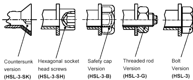
FIGURE 2—HSL-3 HEAD CONFIGURATIONS
