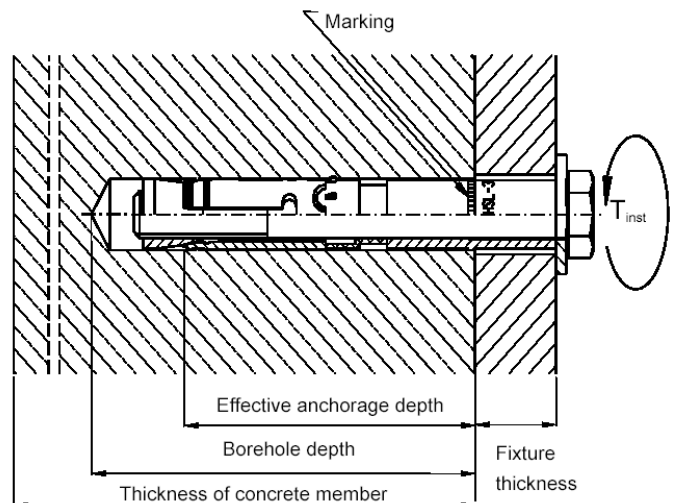
FIGURE 3—CORRECT INSTALLATION OF HSL-3
